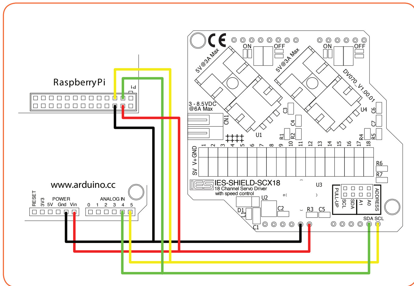
Figure 2.0 (Connection Schematic for Arduino UNO or Raspberry-Pi I 2 C communication)
