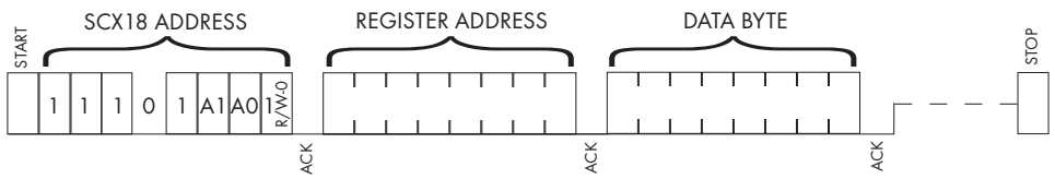
Figure 1.0 (I 2 C write protocol)
